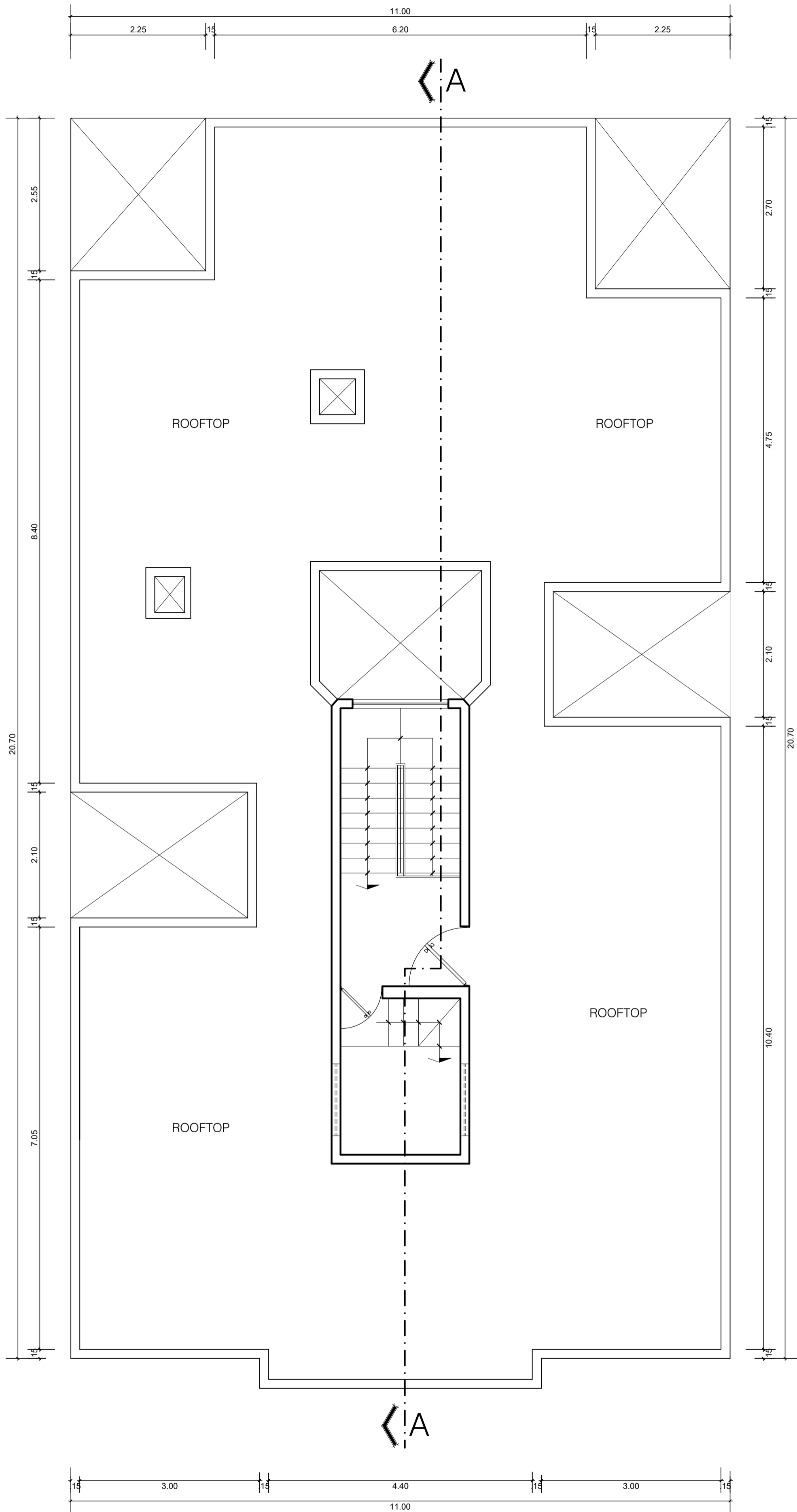
ROOFTOP PLAN SCALE 1/50
